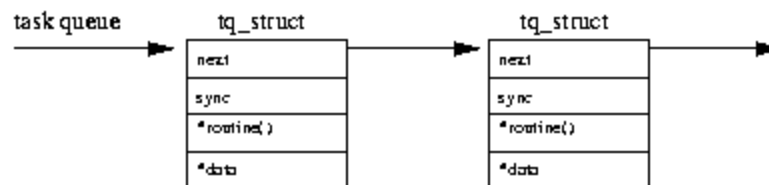
Figure 11.2: A Task Queue
