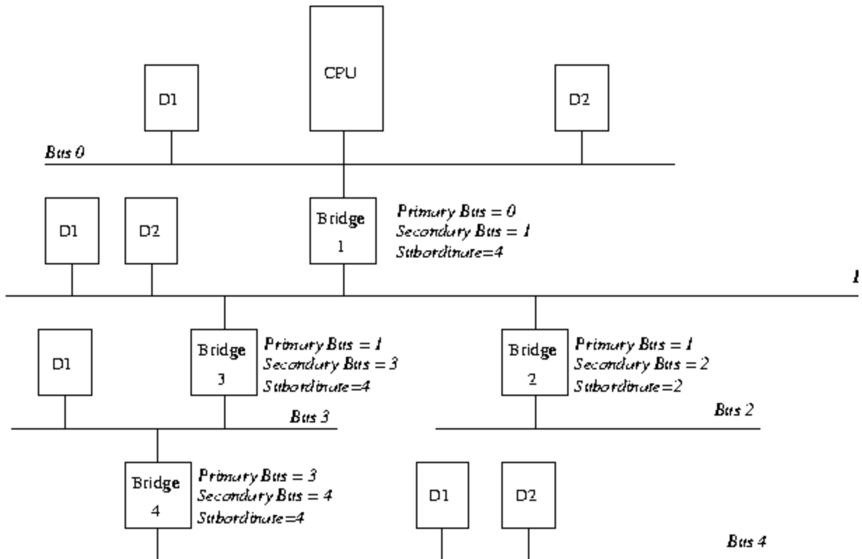
Figure 6.9: Configuring a PCI System: Part 4
