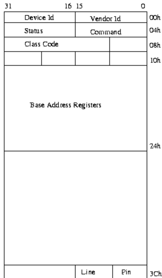
Figure 6.2: The PCI Configuration Header
