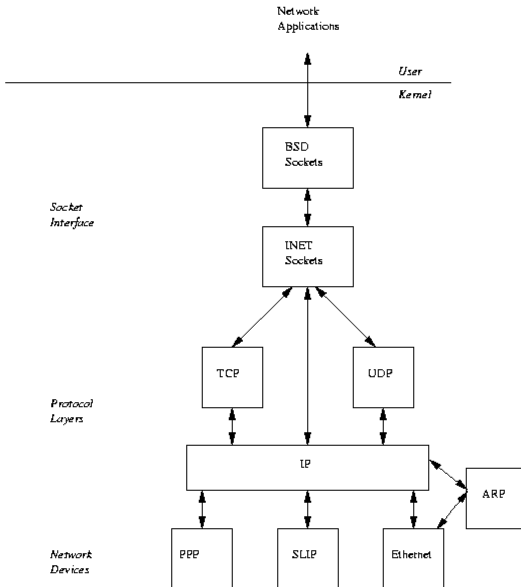
Figure 10.2: Linux Networking Layers
