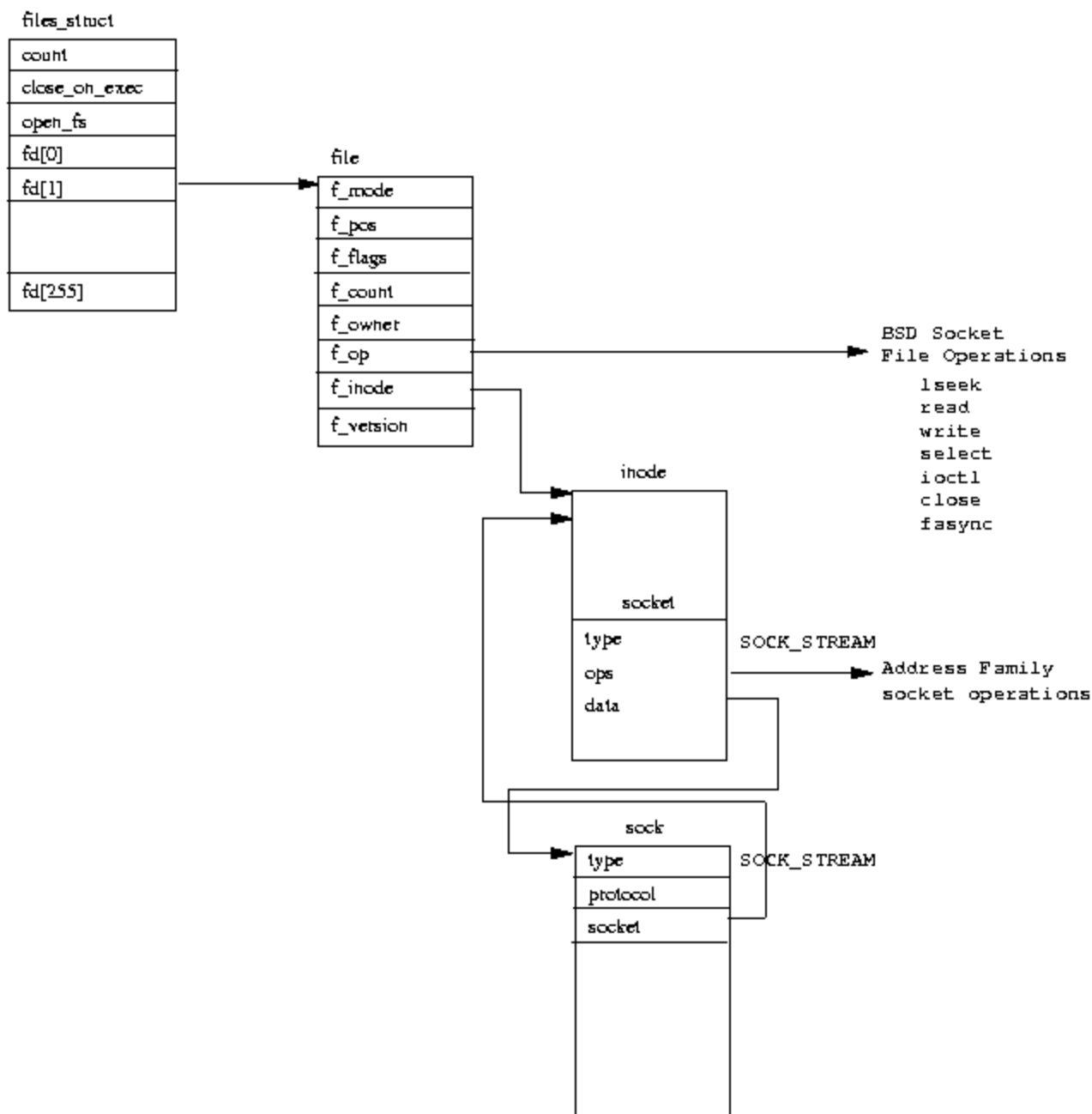
Figure 10.3: Linux BSD Socket Data Structures
