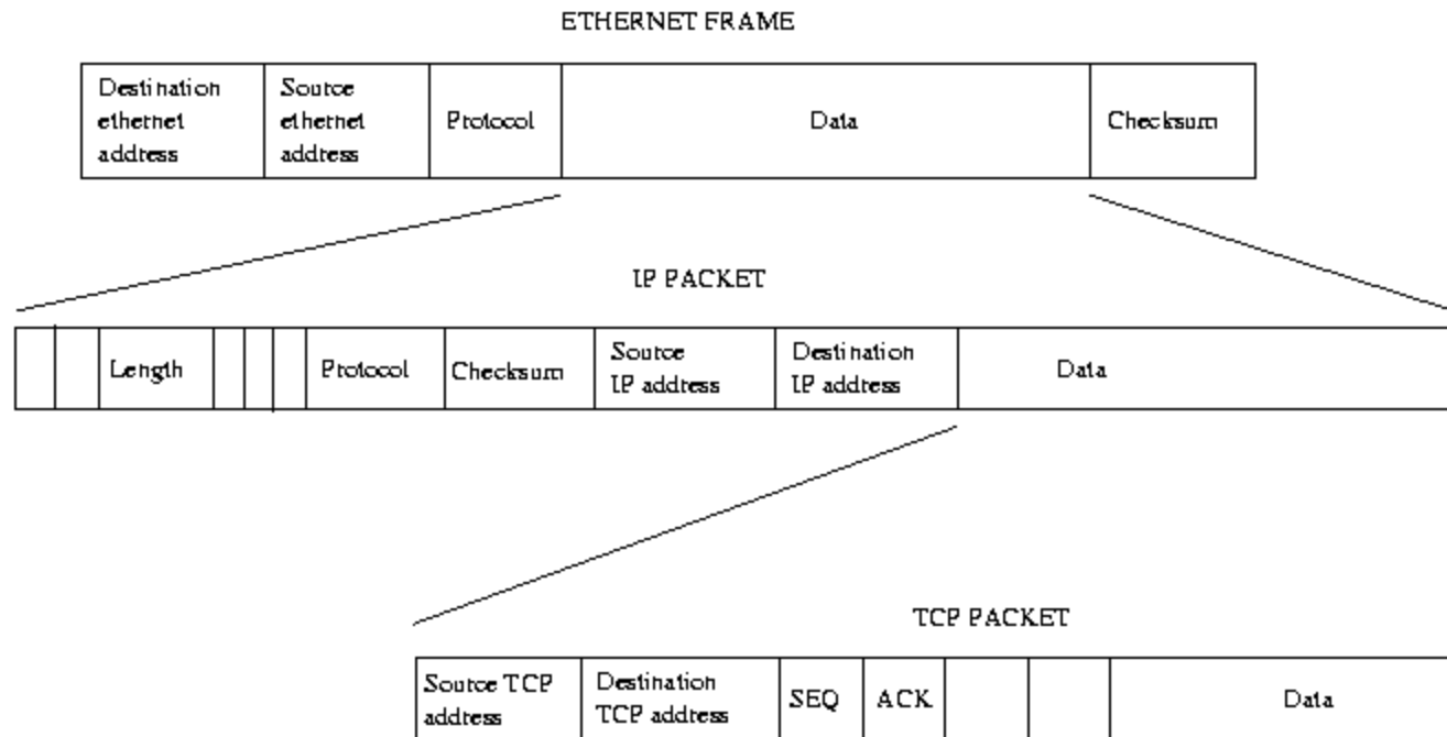
Figure 10.1: TCP/IP Protocol Layers
