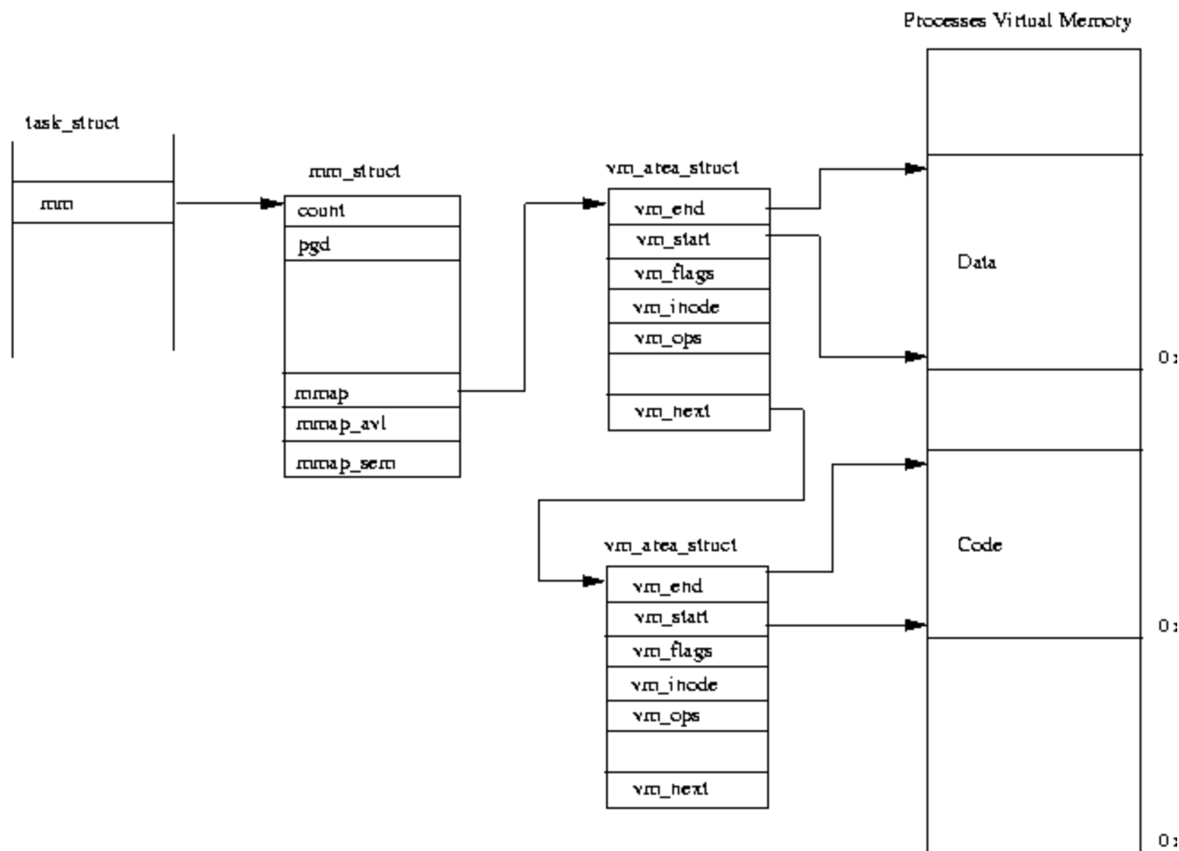
Figure 4.2: A Process's Virtual Memory
