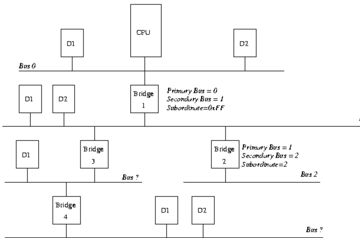
Figure 6.7: Configuring a PCI System: Part 2
