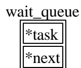
Figure 11.4: Wait Queue
