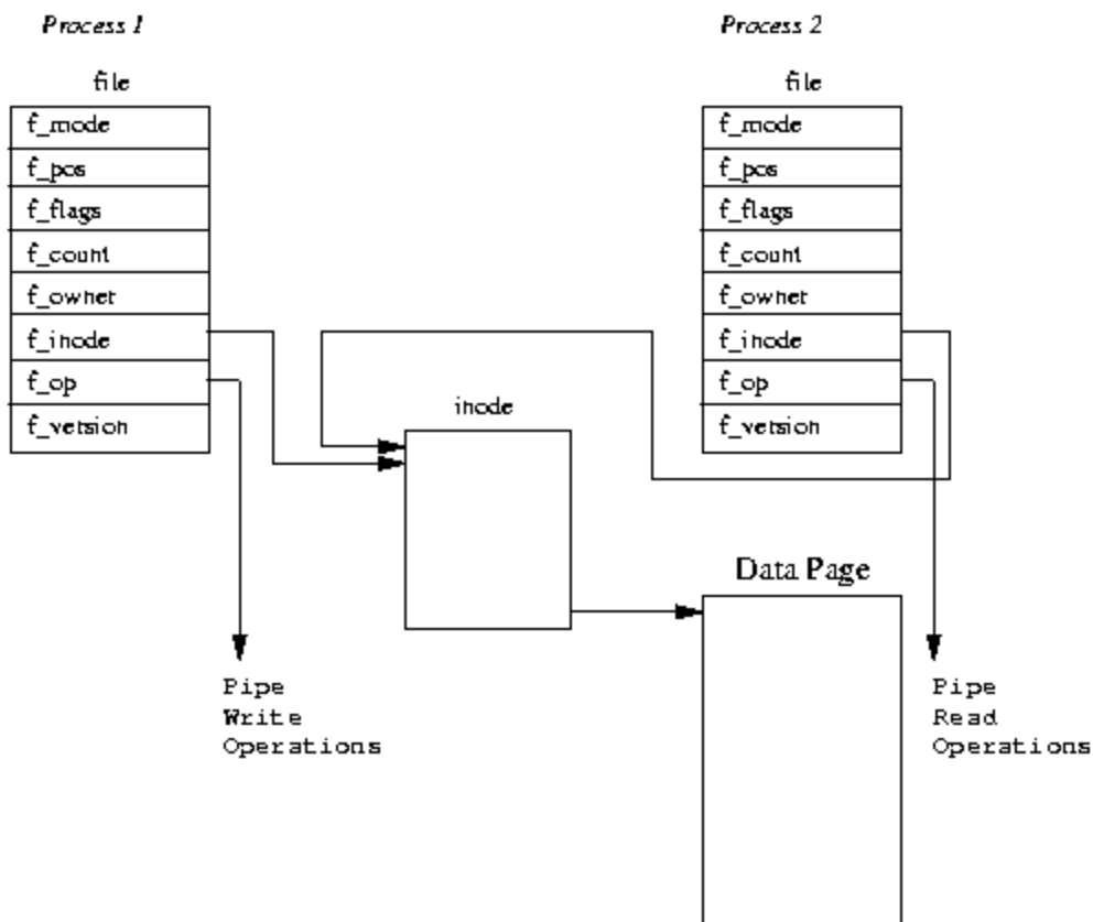
Figure 5.1: Pipes
