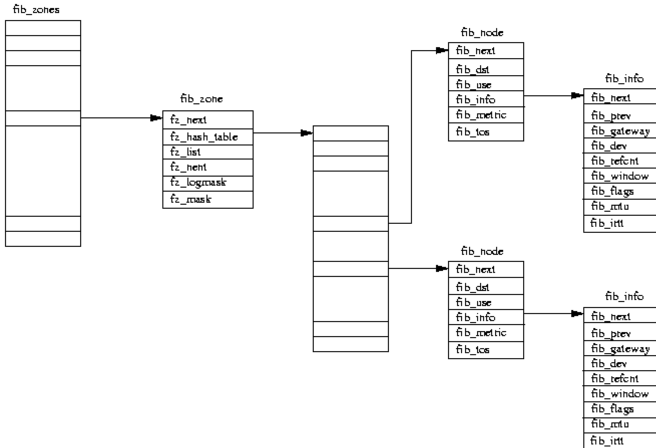
Figure 10.5: The Forwarding Information Database
