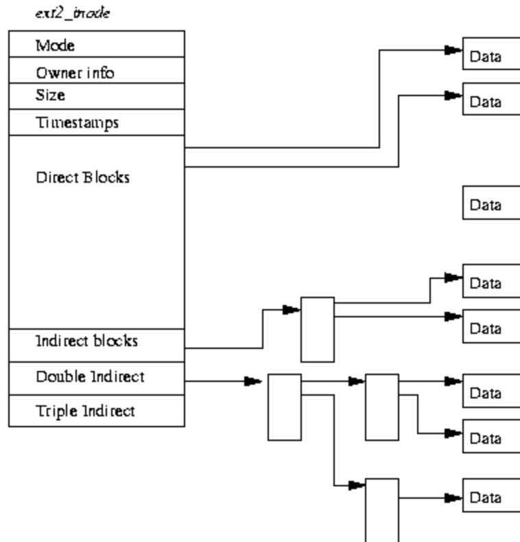
Figure 9.2: EXT2 Inode
