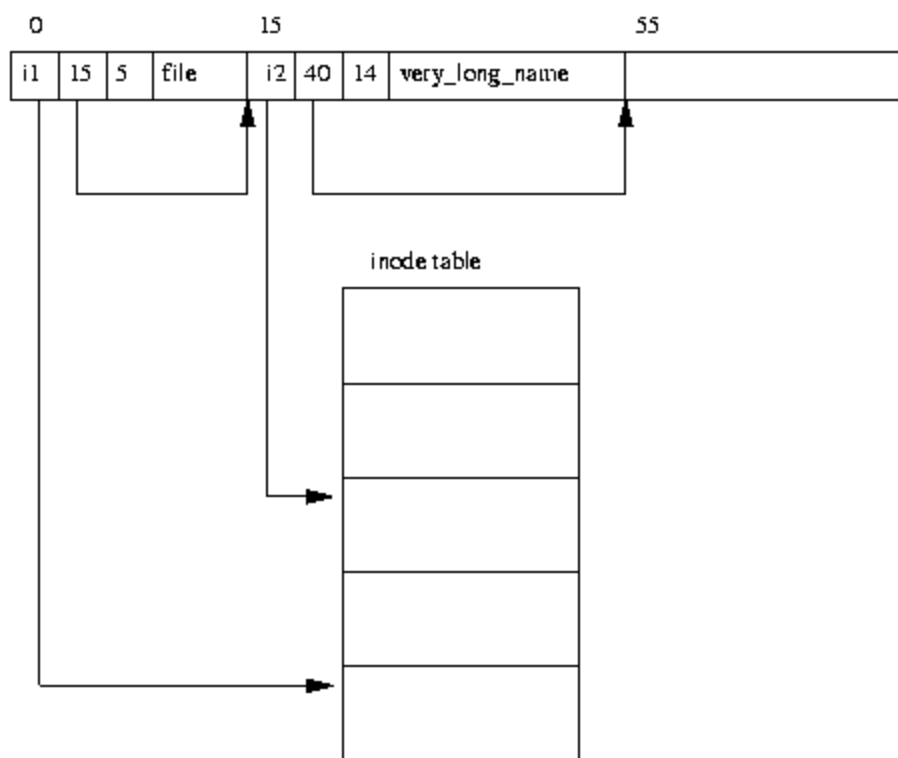
Figure 9.3: EXT2 Directory
