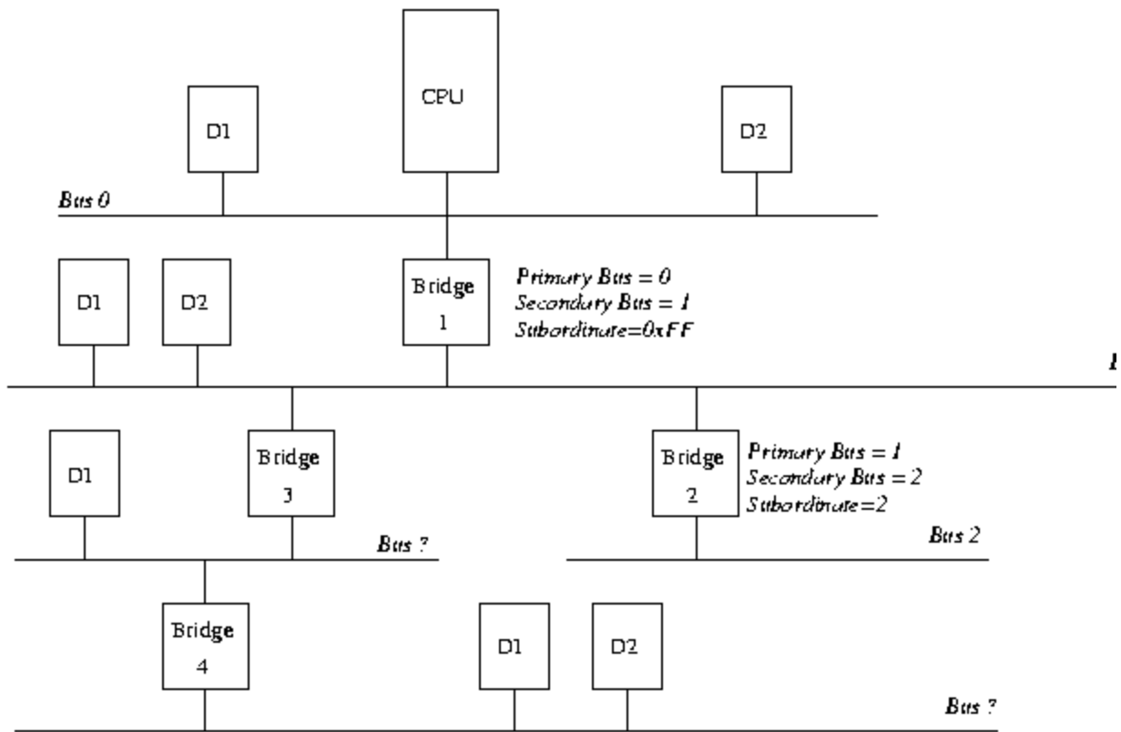
Figure 6.7: Configuring a PCI System: Part 2
