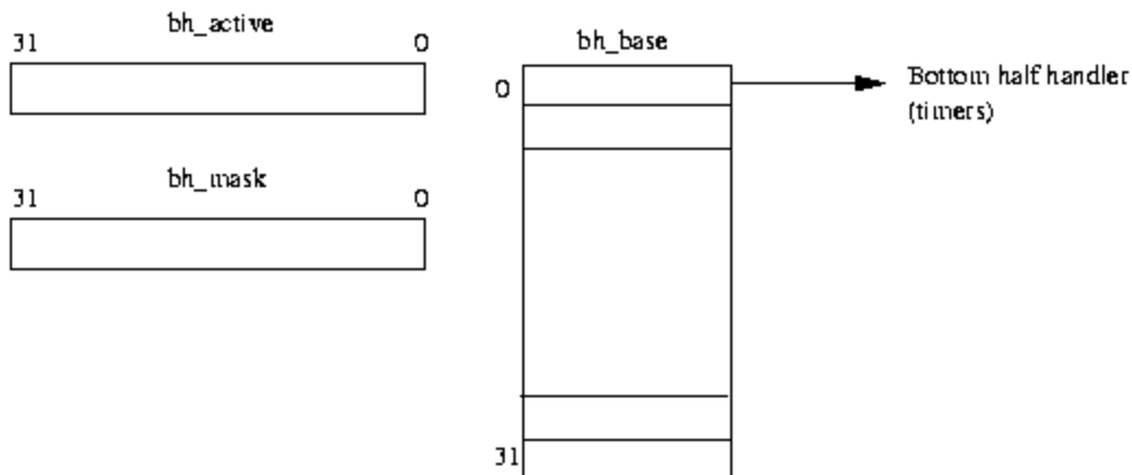
Figure 11.1: Bottom Half Handling Data Structures
