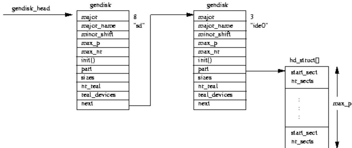
Figure 8.3: Linked list of disks
