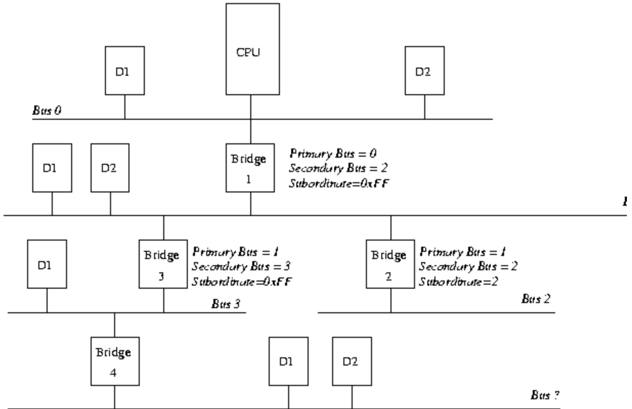
Figure 6.8: Configuring a PCI System: Part 3
