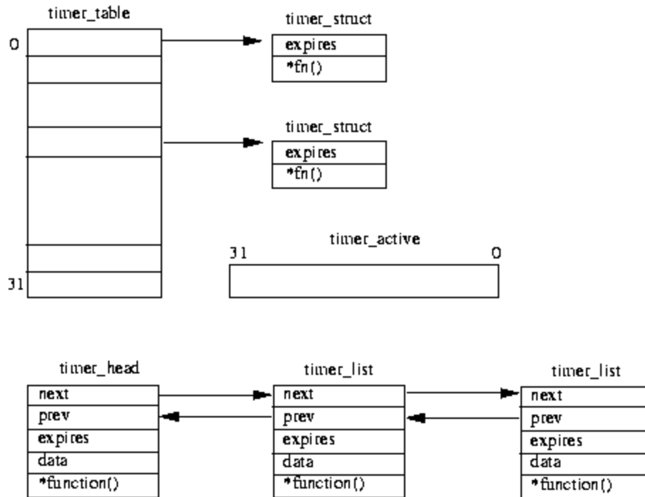
Figure 11.3: System Timers
