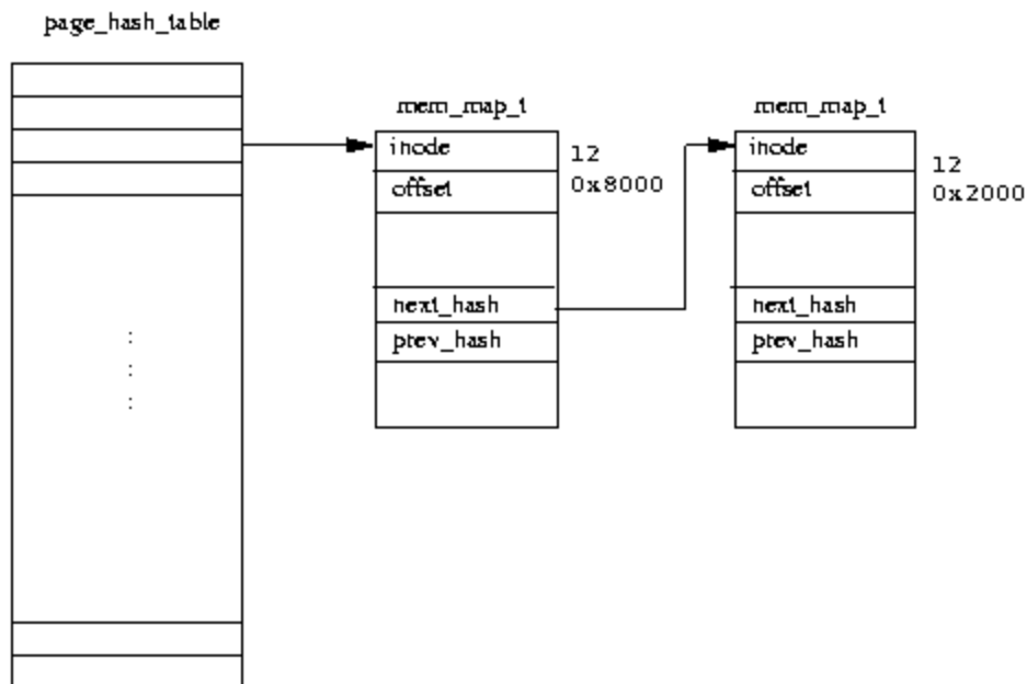
Figure 3.6: The Linux Page Cache
